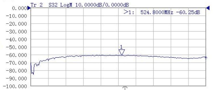
Isolation
