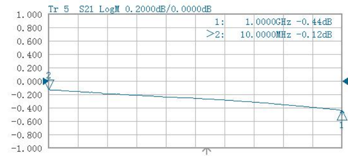
Insert loss
